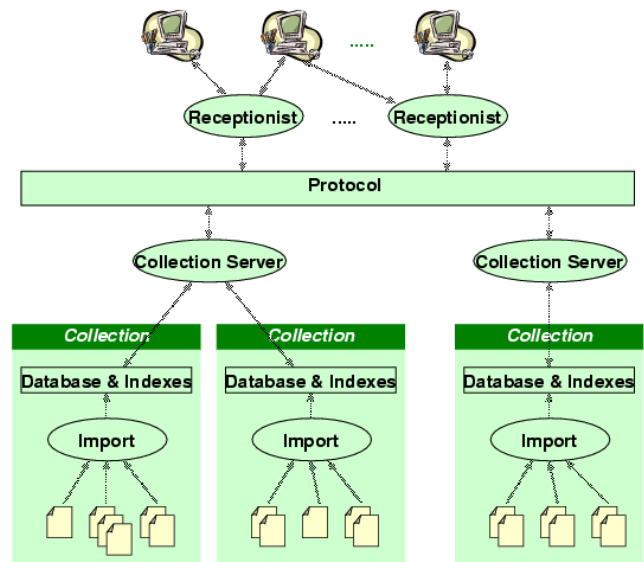
Figure 2: Digital library software architecture
