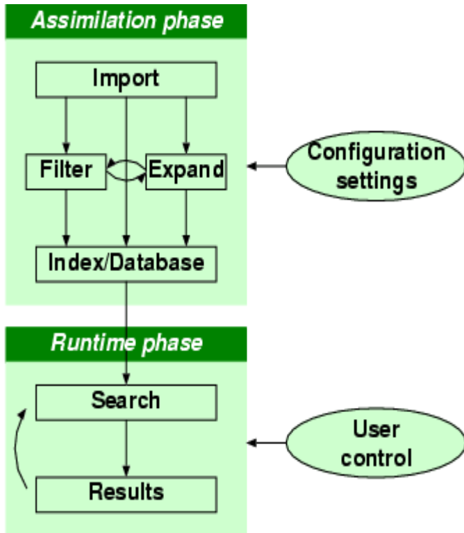
Figure 1: A workbench for symbolic music information retrieval
